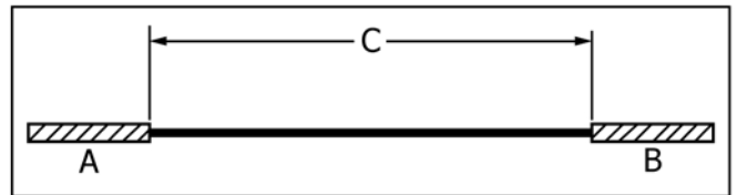
FIG. X5.1 Resistance Areas
